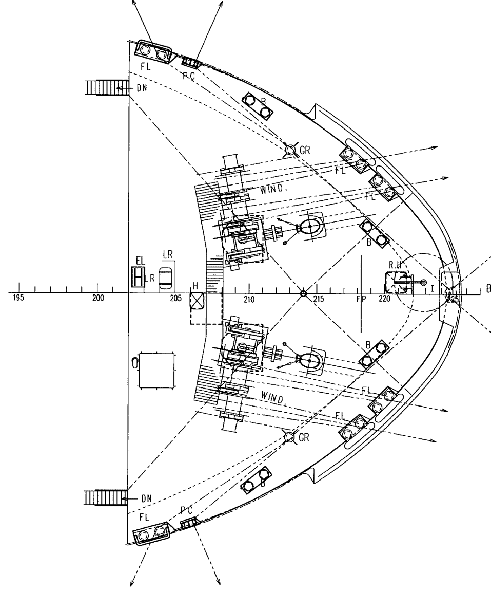
UPPER DECK
