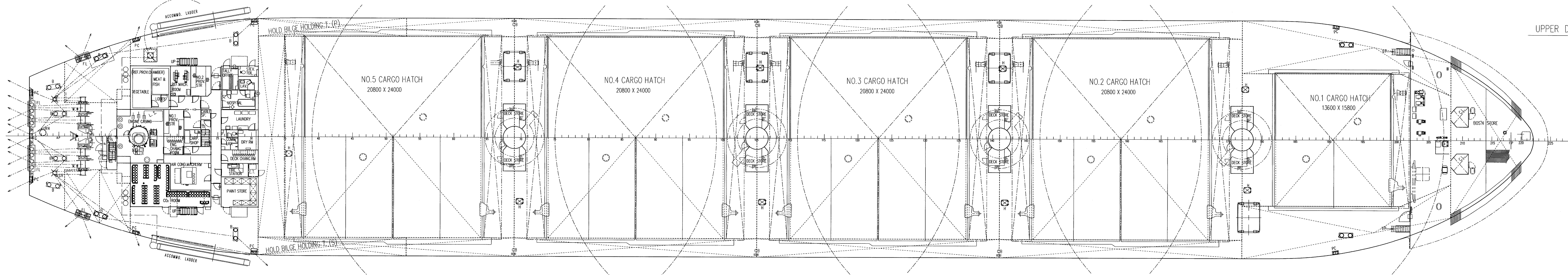
HOLD PLAN
